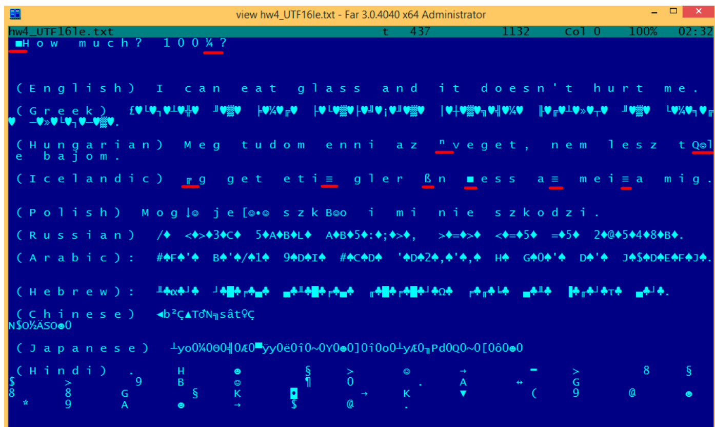
Рис. 5.6: FAR: UTF-16LE
