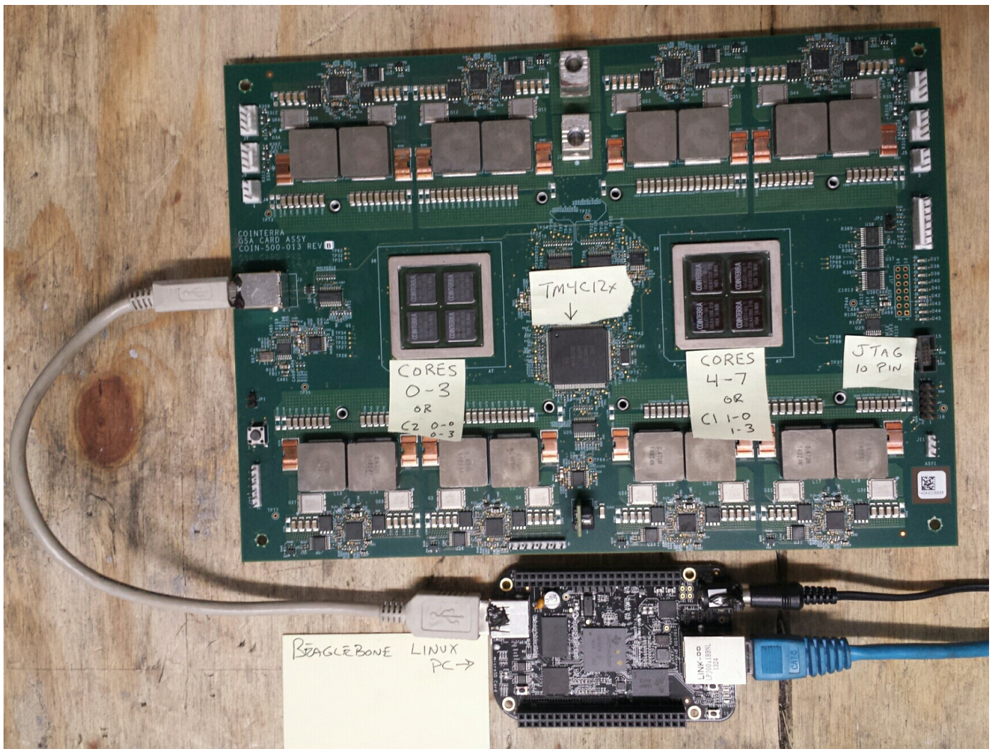
Рис. 8.14: Board
